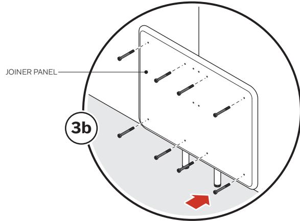
Screw M6 X 50mm Partial Socket, Black (0003010)
