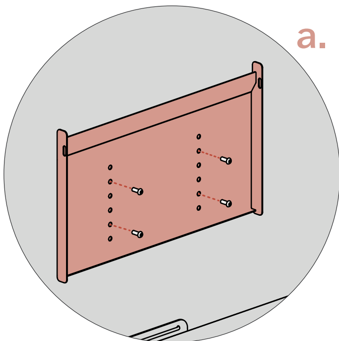
BHSCS M6-1.0 x 16mm Black (125278)
