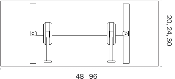
Rectangle Inset Base
